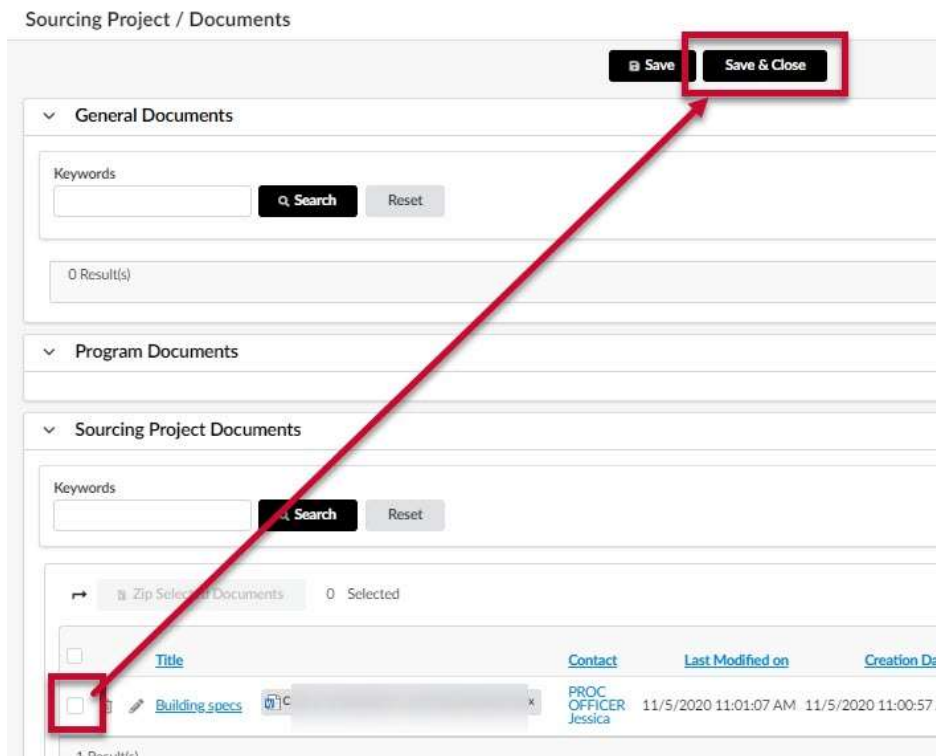
Figure 25: The checkbox for an existing document and the Save & Close button in the Sourcing Project/Documents window.
